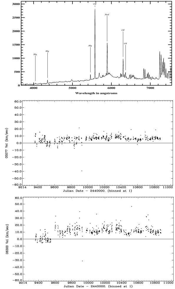
Fig. 25.— emsao reduction of night sky lines from FAST. The top panel shows a typical night sky spectrum, with the lines marked. The middle panel shows the apparent velocity of O[ I ] 5577Å as a function of observation date. Each point is the nightly median, where nights with fewer than 10 observations are excluded. The bottom panel is similar to the middle, but shows the apparent velocity of the O[ I ] 6300Å line. Note that the scale of the ordinate is half that in figure 24
