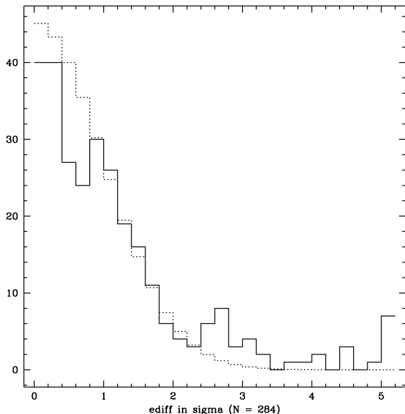
Fig. 5.— The solid histogram is the distribution of velocity differences for duplicate observations of the same object, reduced with the emtemp template, divided by the xcsao error estimate. The dotted histogram is the expected Gaussian.
