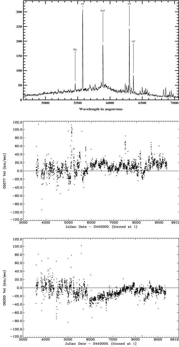
Fig. 24.— emsao reduction of night sky lines from the Z-Machine. The top panel shows a typical night sky spectrum, with the lines marked. The middle panel shows the apparent velocity of O[ I ] 5577Å as a function of observation date. Each point is the nightly median, where nights with fewer than 10 observations are excluded. The bottom panel is similar to the middle, but shows the apparent velocity of the O[ I ] 6300Å line.
