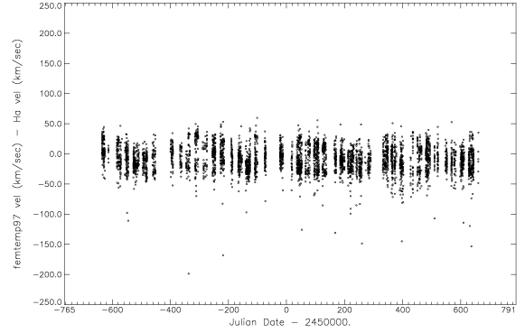
Fig. 22.— The difference between velocities obtained by fitting H \alpha and correlating with the femtemp97 template, for 4833 spectra where r > 5 and H \alpha was fit, as a function of observation date.
