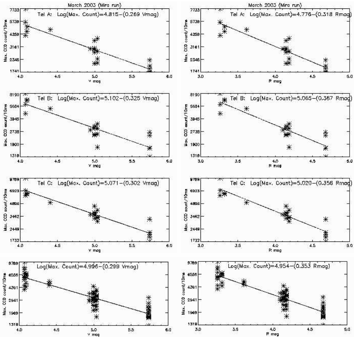
Fig.3: Maximum CCD counts are plotted against V magnitudes (left) and R magnitudes (right) for all three telescopes. Top three rows correspond to Telescope A, B & C respectively and the bottom row shows all three telescope data together.
