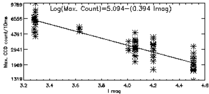
Fig.2: Same as figure 1, but all three telescope values are used together. A least square fit to the data and the best fit parameters are given.
