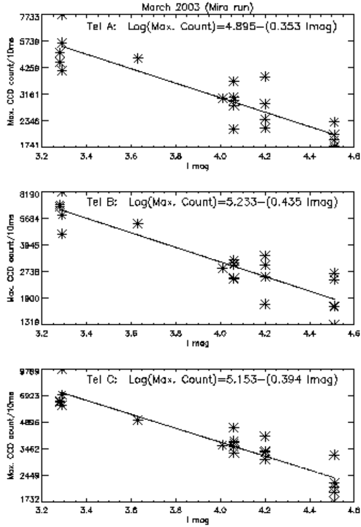
Fig.1: Maximum CCD counts are plotted against I magnitudes for all three telescopes. A least square fit to the data are shown and the best fit parameters are given.
