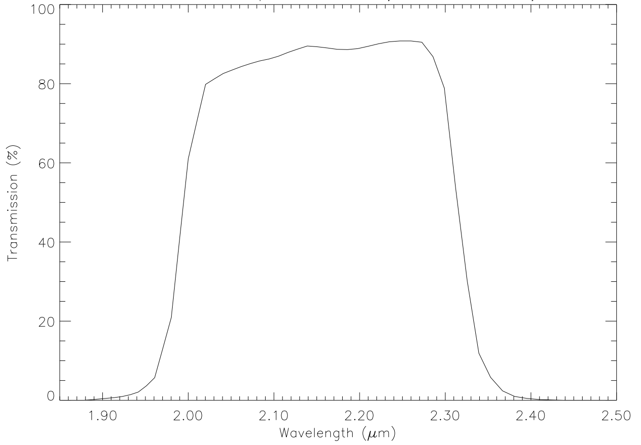
IOTA Filter - K-prime, \lambda_c=2.16\mu\text{m} , FWHM= 0.32\mu\text{m}
