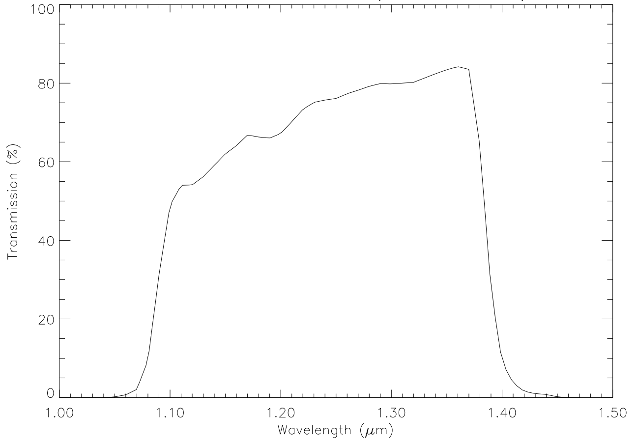
IOTA Filter – J Band, \lambda_c=1.25\mu\text{m} , FWHM= 0.29\mu\text{m}
