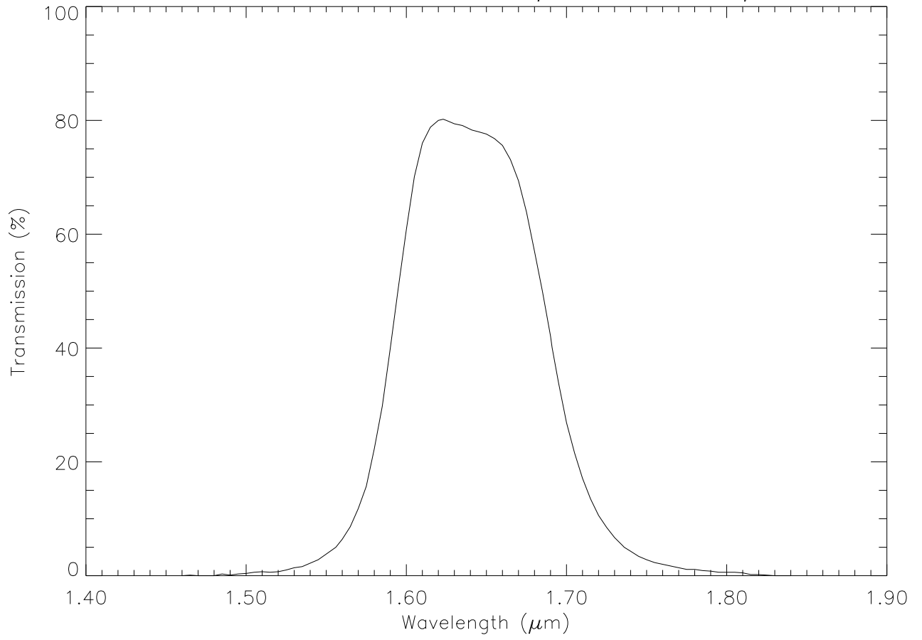
IOTA Filter – H164, \lambda_c=1.64\mu\text{m} , FWHM= 0.10\mu\text{m}
