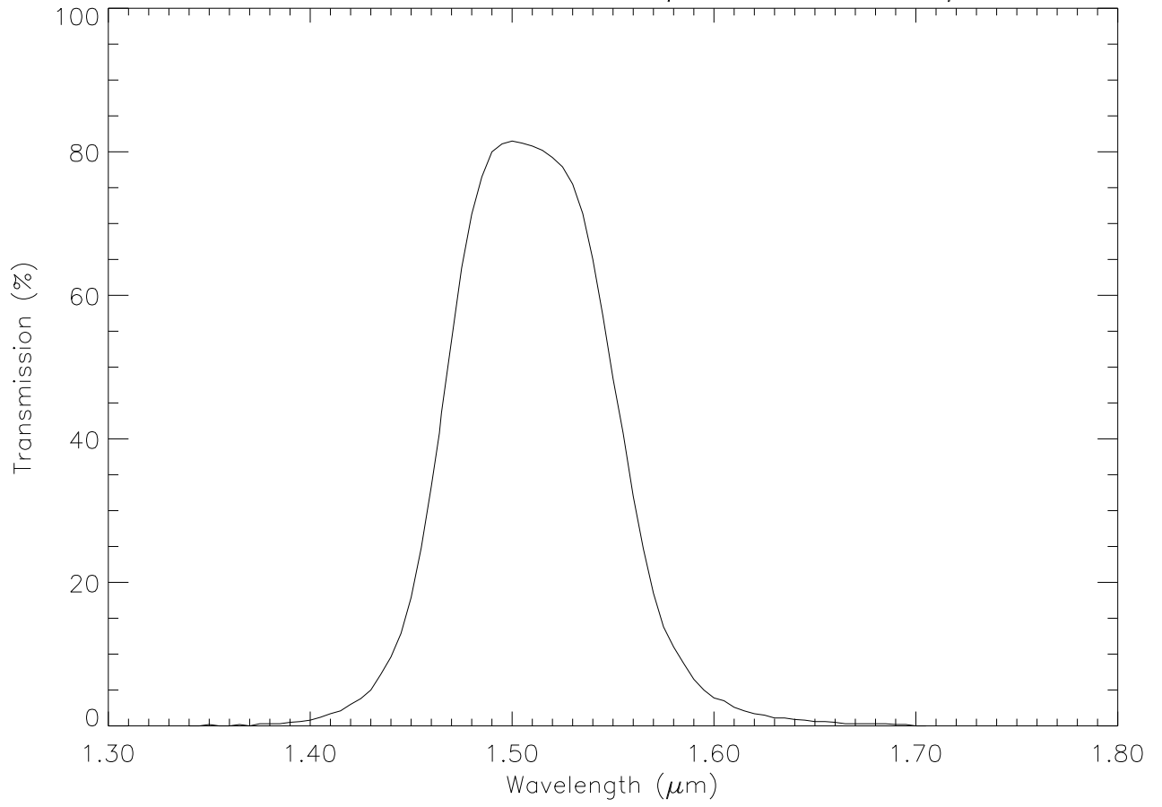
IOTA Filter - H151, \lambda_c=1.51\mu\text{m} , FWHM=0.091 \mu\text{m}
