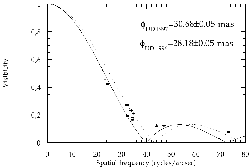
Fig. 1. Fit of the 1996 and 1997 data by uniform disk models. Full circles: 1996 data. Open circles: 1997 data.
