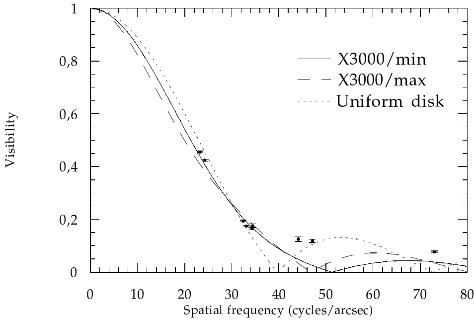
Fig. 2. Fit of the 1997 data by the X3000 Mira model. Continuous line: X3000/min model. Dashed line: X3000/max model. Dotted line: uniform disk model.
