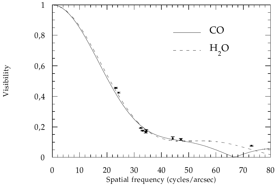
Fig. 6. Fit of the 1997 data by CO and H 2 O intensity profiles of the X3000/max model.
