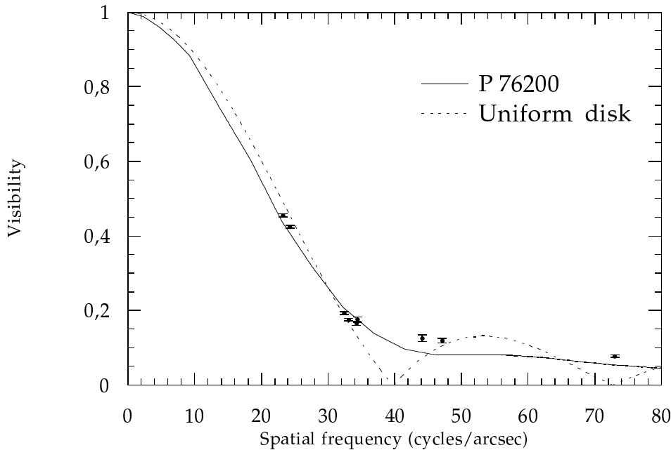
Fig. 4. Fit of the 1997 data by the P 76200 Mira model.
