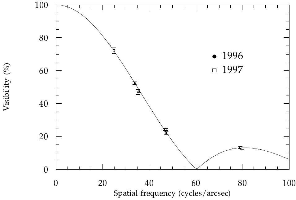
Fig. 5. Visibilities measured on \alpha Bootis in 1996 and 1997. Full circles are the 1996 data points. Open squares are the 1997 data points. The continuous line is a uniform disk model fit of the 1996 data. The 1997 data points are fully consistent with the 1996 model and no variation of diameter is detected for this reference star.
