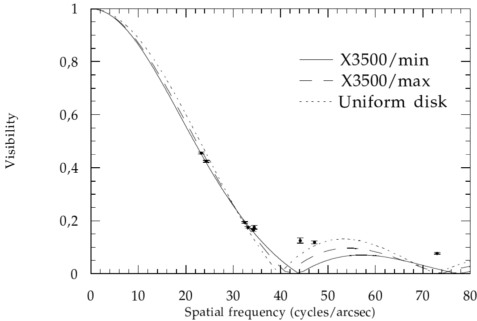
Fig. 3. Fit of the 1997 data by the X3500 Mira model. Continuous line: X3500/min model. Dashed line: X3500/max model. Dotted line: uniform disk model.
